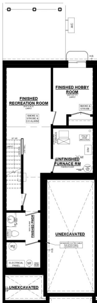
ASHTON 'C' UNIT #3 BASEMENT PLAN 415 SQ. FT. FINISHED BASEMENT SPACE
