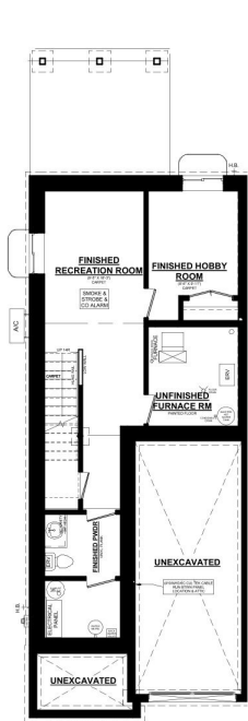
ASHTON C UNIT #1 BASEMENT PLAN 415 SQ. FT. FINISHED BASEMENT SPACE
