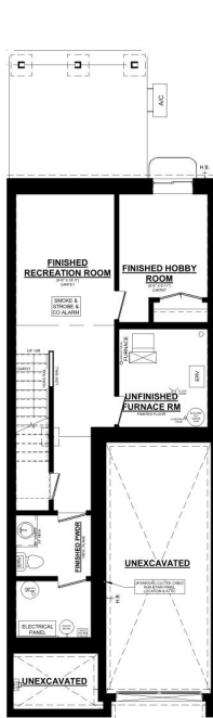
Ashton C UNIT #3 BASEMENT PLAN 415 SQ. FT. FINISHED BASEMENT SPACE
