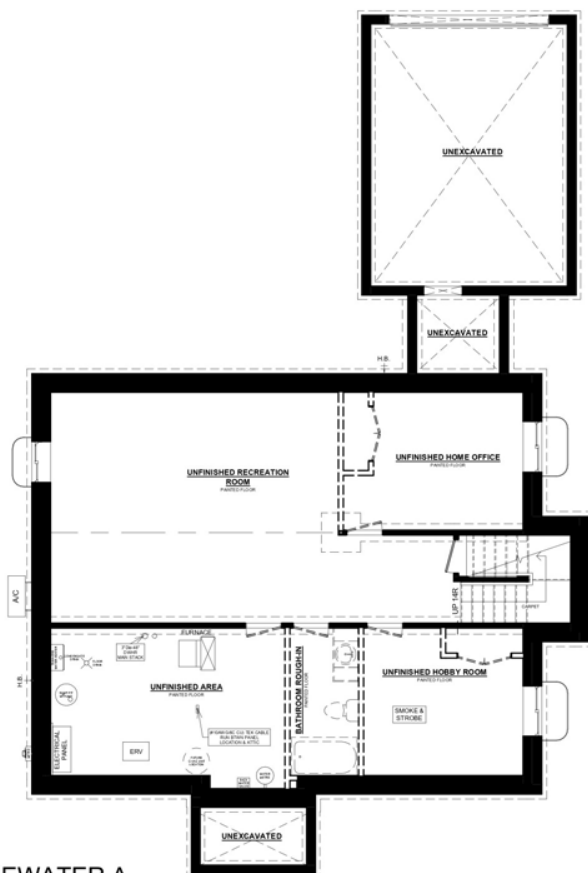
BRIDGEWATER A UNFINISHED BASEMENT PLAN
