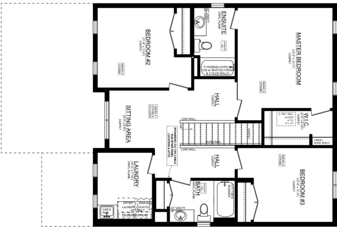
OAKMONT 'C' 2ND FLOOR PLAN 1057 SQ. FT. 8' CEILING ON 2ND FLOOR
