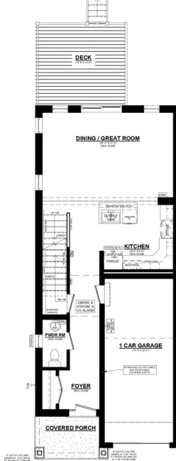
ASHTON 'A' UNIT #1 END MAIN FLOOR PLAN 690 SQ. FT. 8' CEILINGS ON MAIN FLOOR
