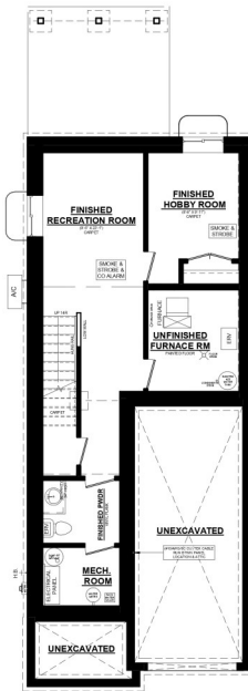
ASHTON 'A' UNIT #1 END BASEMENT PLAN 415 SQ. FT. FINISHED BASEMENT SPACE
