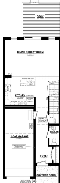
ASHTON 'A' UNIT #4 INT MAIN FLOOR PLAN 660 SQ. FT. 8' CEILINGS ON MAIN FLOOR
