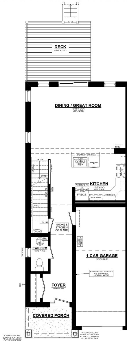
ASHTON 'A' UNIT #1 END MAIN FLOOR PLAN 690 SQ. FT. 8' CEILINGS ON MAIN FLOOR
