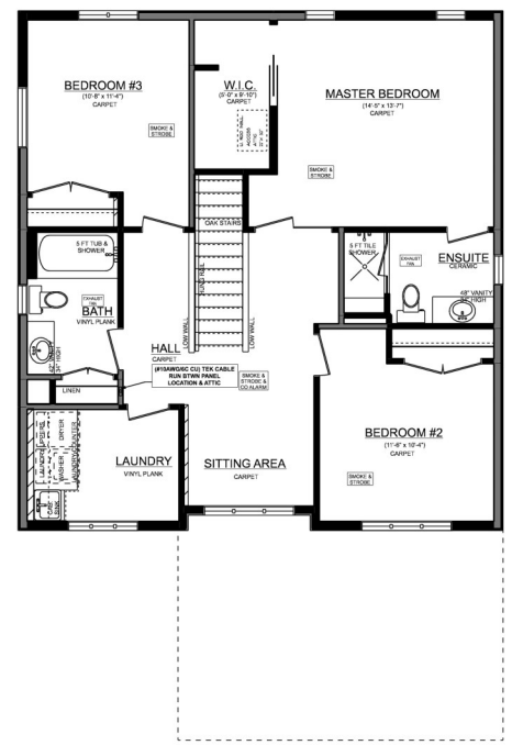
OAKMONT 'A' 2ND FLOOR PLAN 1044 SQ. FT. 8' CEILING ON 2ND FLOOR
