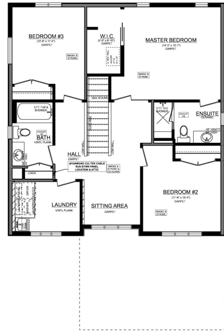
OAKMONT 'A' 2ND FLOOR PLAN 1044 SQ. FT. 8' CEILING ON 2ND FLOOR
