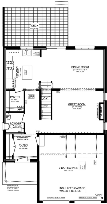
OAKMONT 'A' MAIN FLOOR PLAN 948 SQ. FT. 8' CEILING ON MAIN FLOOR
