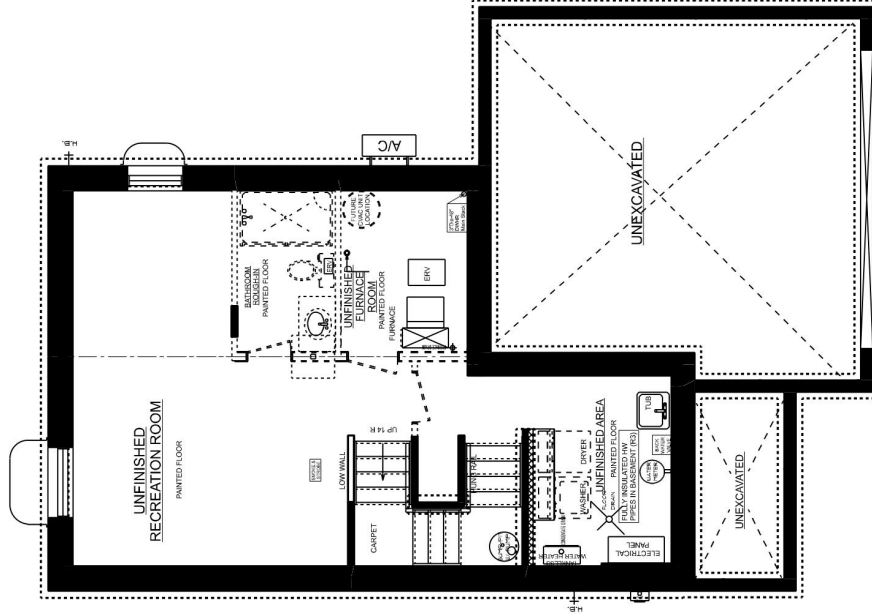
ASPEN 'B' BASEMENT PLAN 2 CAR
