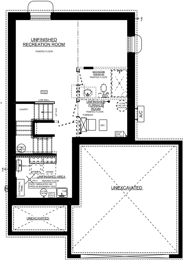
ASPEN 'B' BASEMENT PLAN 2 CAR
