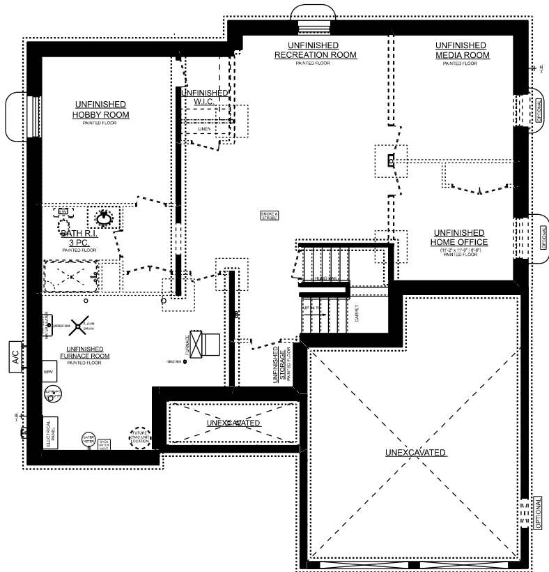
SOMERDALE 'A' BASEMENT PLAN
