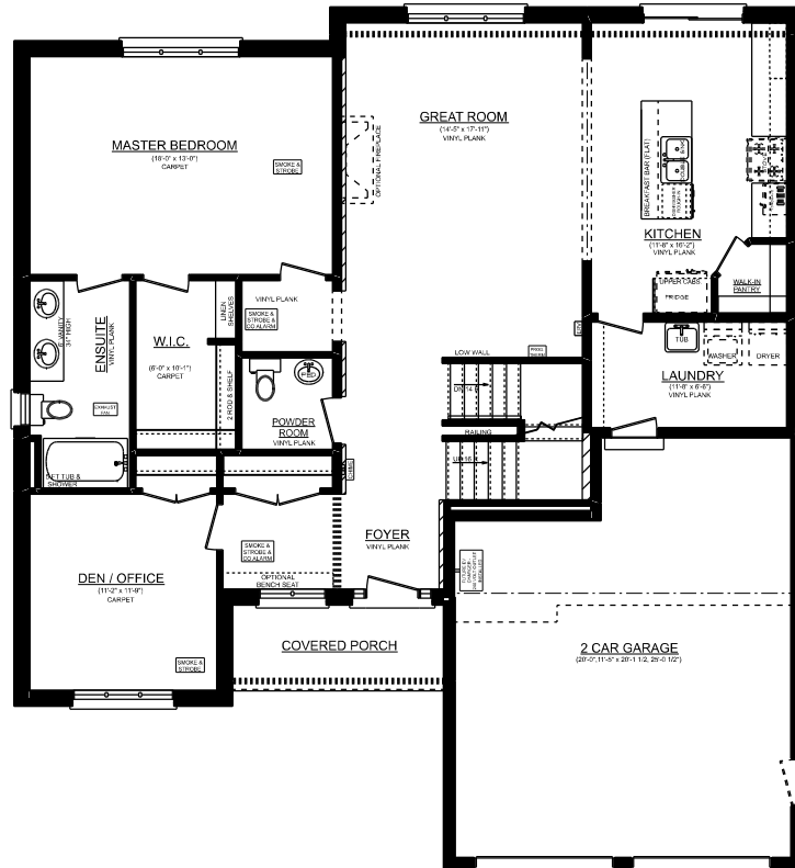
SOMERDALE 'A' MAIN FLOOR 1537 SQ. FT. 9' CEILINGS ON MAIN FLOOR
