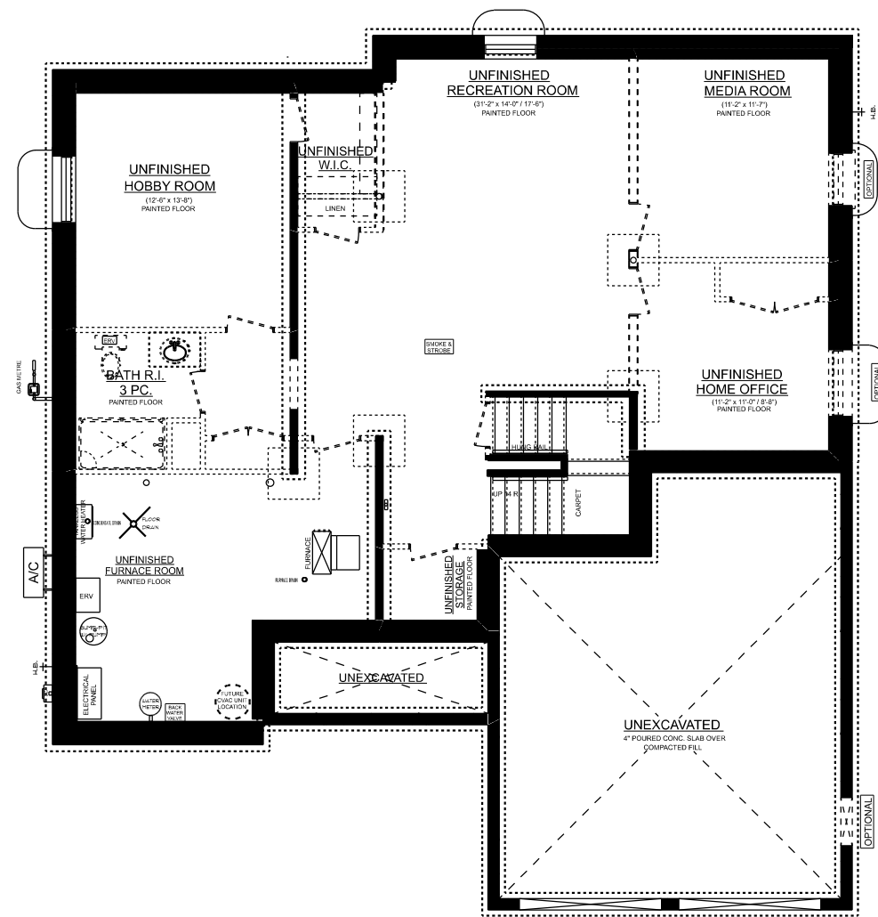
SOMERDALE 'A' BASEMENT PLAN
