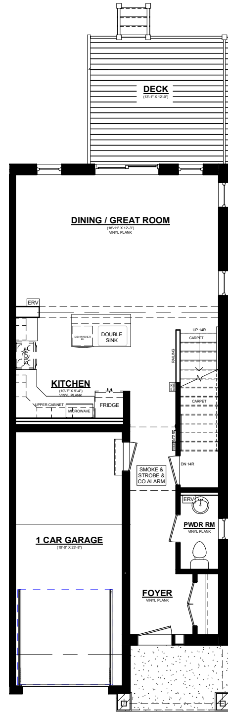
Ashton B UNIT #5 MAINFLOOR PLAN 690 SQ. FT. 8' CEILINGS ON MAINFLOOR' CEILINGS ON MAINFLOOR
