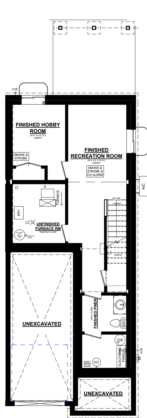
Ashton B UNIT #5 BASEMENT PLAN 378 SQ. FT. FINISHED BASEMENT SPACE
