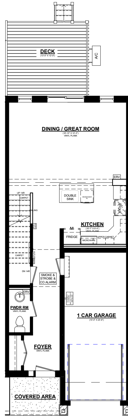
Ashton B UNIT #4 MAINFLOOR PLAN 690 SQ. FT. 8' CEILINGS ON MAINFLOOR' CEILINGS ON MAINFLOOR
