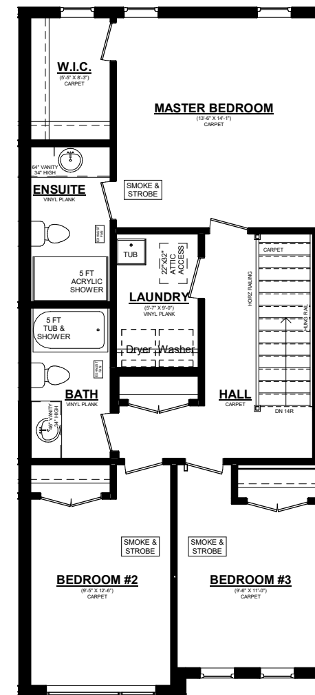
Ashton B UNIT #4 2ND FLOOR PLAN PLAN 910 SQ. FT. 8' CEILINGS ON 2ND FLOOR' CEILINGS ON 2ND FLOOR PLAN
