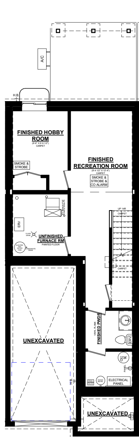
Ashton B UNIT #2 BASEMENT PLAN 378 SQ. FT. FINISHED BASEMENT SPACE
