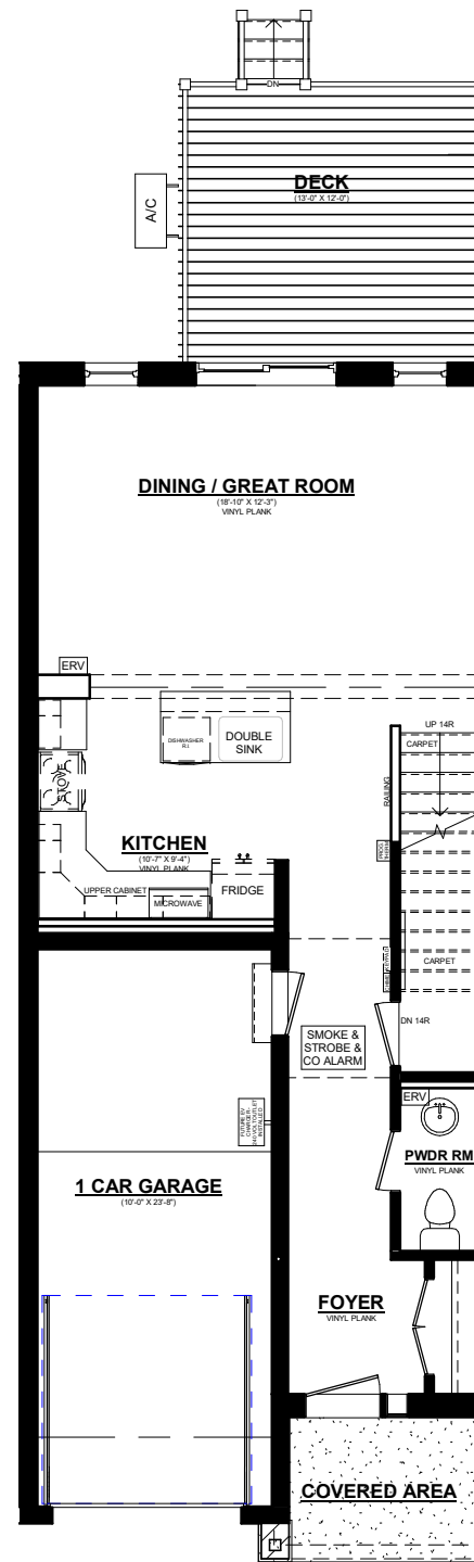
Ashton B UNIT #2 MAINFLOOR PLAN 690 SQ. FT. 8' CEILINGS ON MAINFLOOR' CEILINGS ON MAINFLOOR
