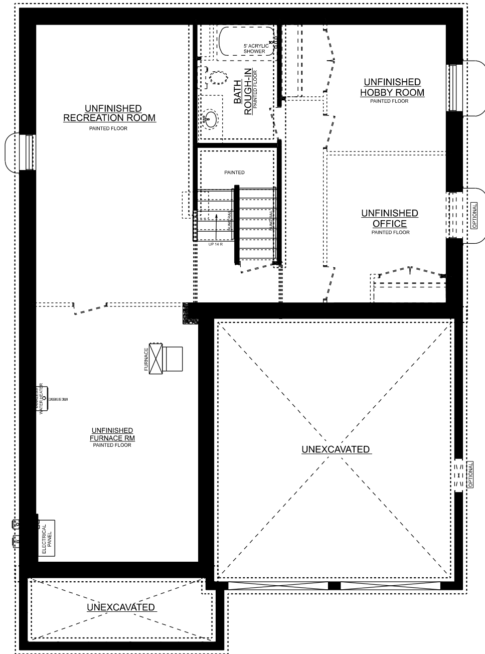
BASEMENT PLAN
