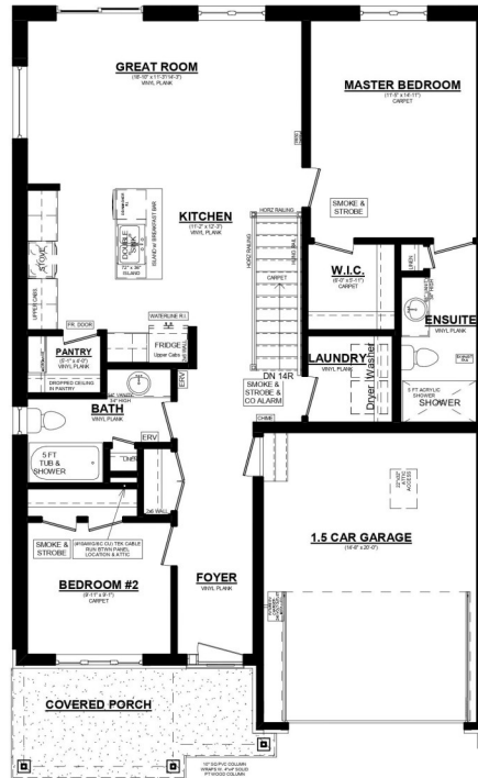
EASTON A UNIT #1 MAINFLOOR PLAN 1200 SQ. FT. 8" CEILINGS ON MAINFLOOR
