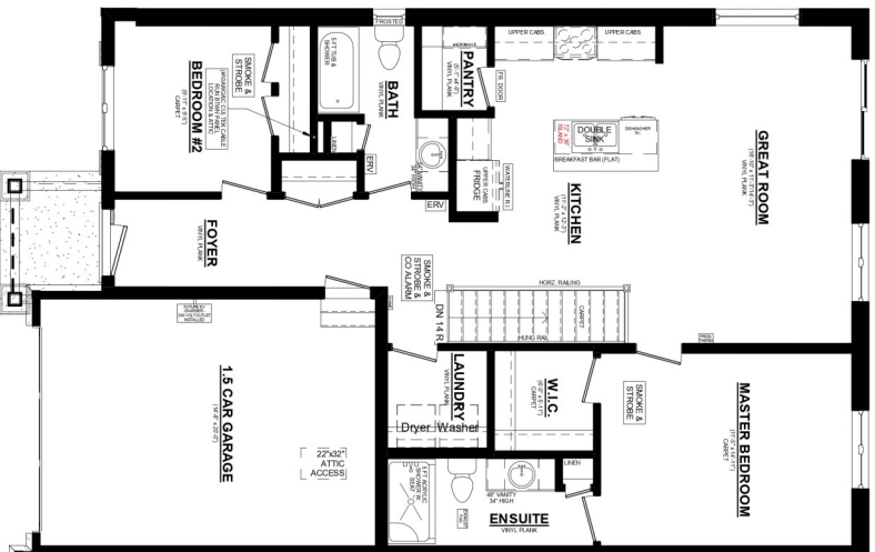
EASTON D UNIT #1 MAIN FLOOR PLAN 1200 SQ. FT. 8' CEILINGS ON MAIN FLOOR
