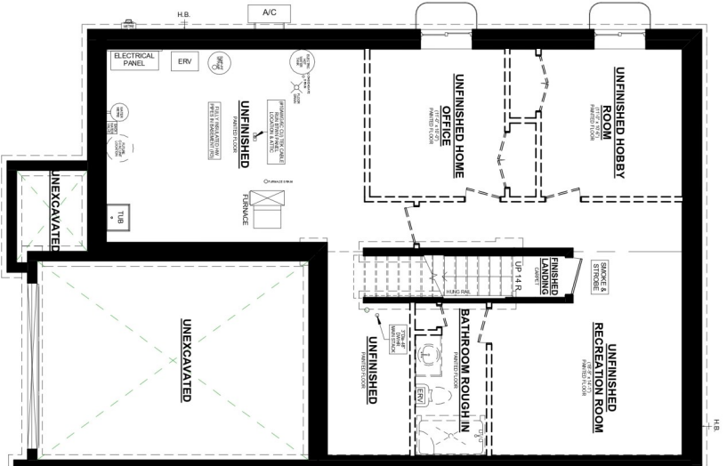
EASTON D UNIT #1 BASEMENT PLAN
