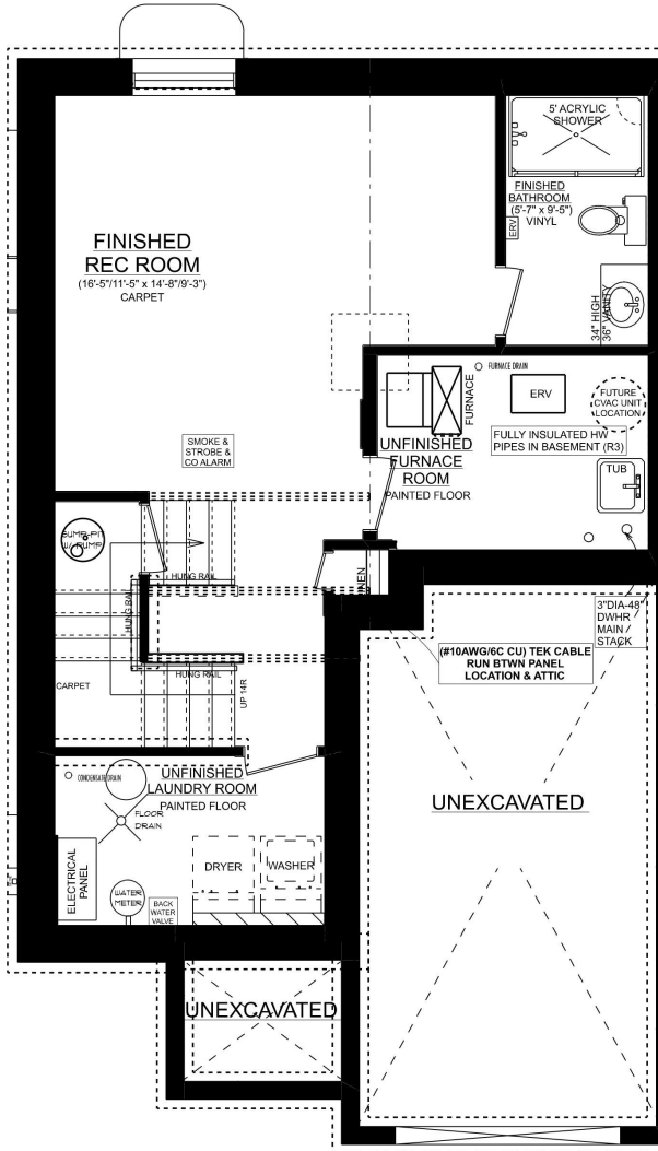
KENSINGTON 'C' UNIT #1 BASEMENT PLAN 320 SQ.FT. FINISHED SPACE
