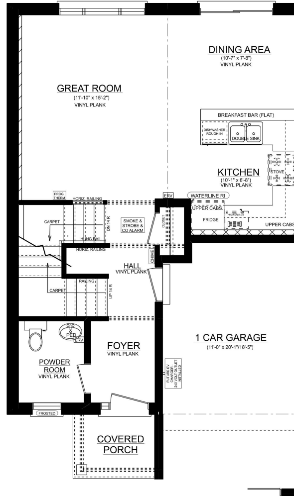
KENSINGTON 'C' UNIT #1 MAINFLOOR PLAN 8' CEILINGS ON MAIN FLOOR 1 CAR 650 SQ. FT.
