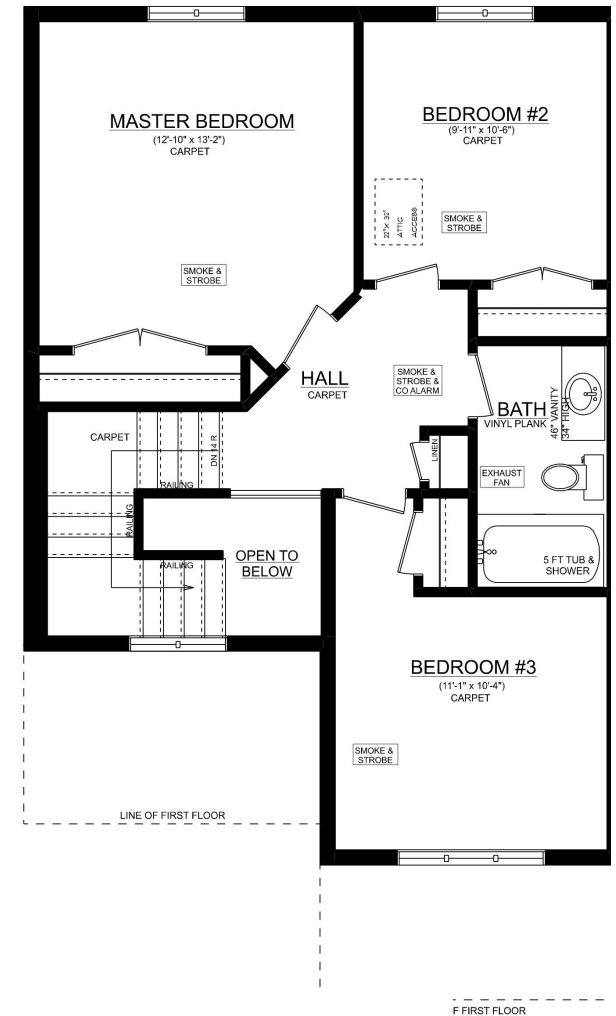
KENSINGTON 'C' UNIT #1 2ND FLOOR PLAN 8' CEILINGS ON 2ND FLOOR 644 SQ. FT. (DOES NOT INCLUDE 87 SQ.FT. OPEN TO BELOW)
