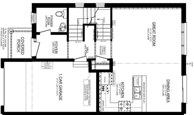
KENSINGTON 'C' UNIT #1 MAIN FLOOR PLAN 8' CEILINGS ON MAIN FLOOR 1 CAR 650 SQ. FT.
