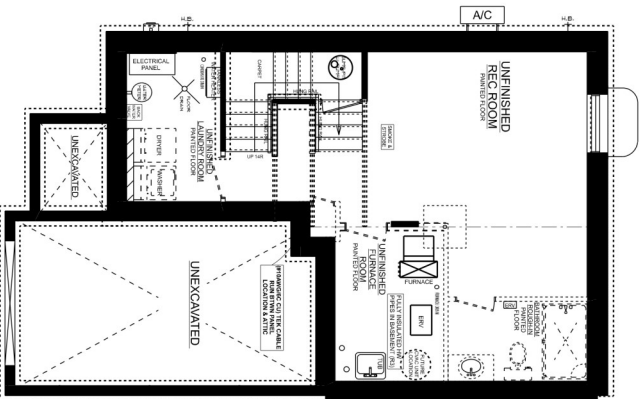
KENSINGTON 'C' UNIT #1 BASEMENT PLAN
