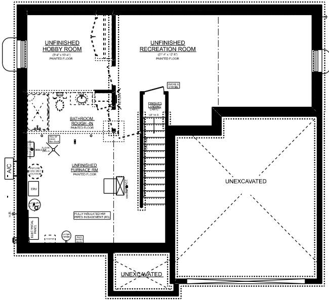
BRIARWOOD 'A' BASEMENT PLAN
