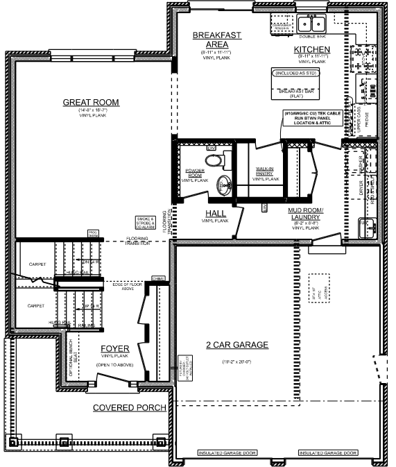
MAINFLOOR PLAN 939 SQ.FT. 8' CEILINGS ON MAINFLOOR
