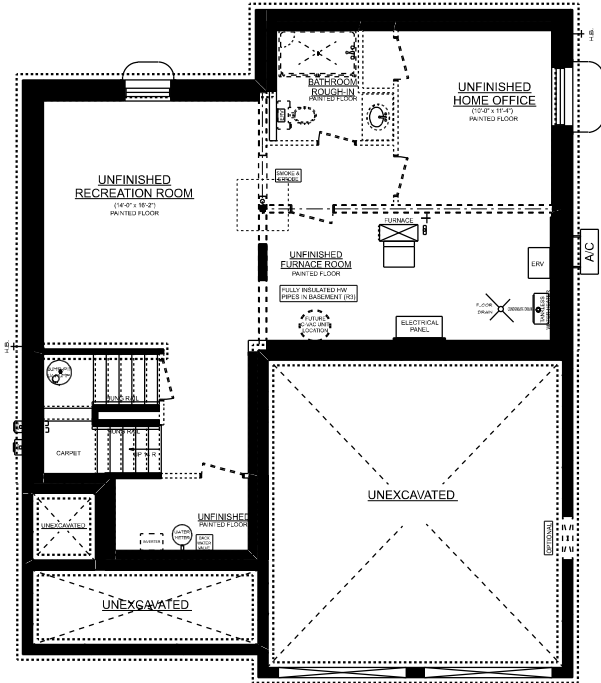
BASEMENT PLAN
